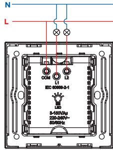
LED dimmer - 1 Way operation
