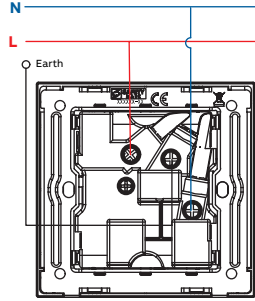
1G 15 A switched socket outlet
