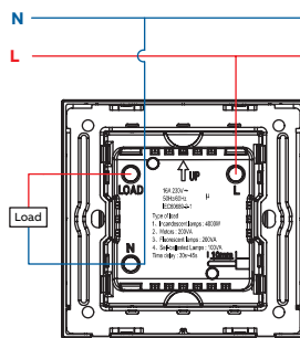
Electronic Card Switch
