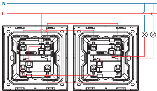
2G 2W switch
