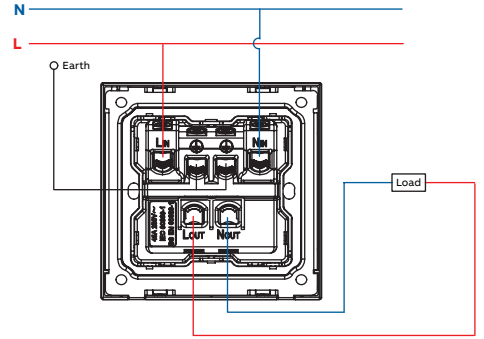
1G 1W switch 32A/45A DP
