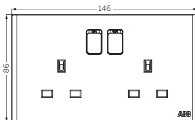
Dimensions for 2gang frames
