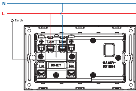
Cooker switch unit
