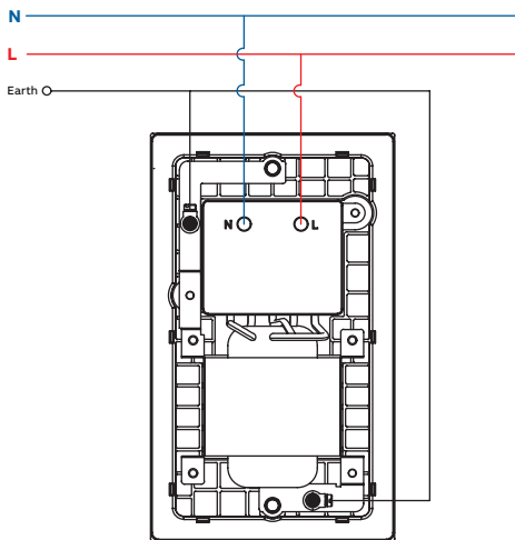
Shaver unit
