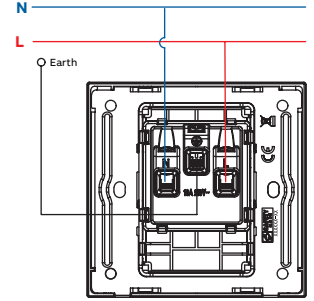
1G/2G 16A Euro-American Socket with Earth
