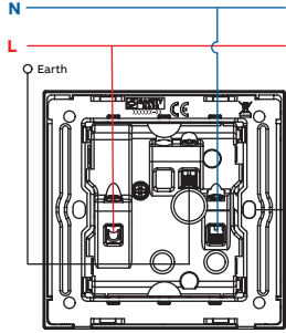
1G 5 A switched socket outlet
