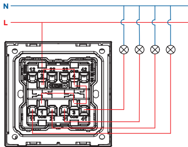
4G 1W switch
