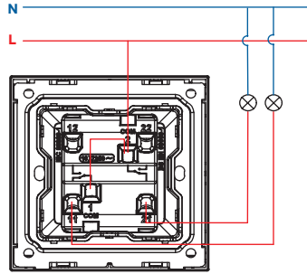
2G 1W switch
