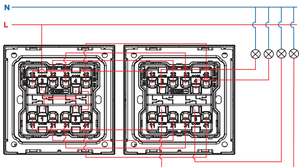
4G 2W switch
