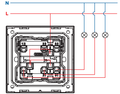
3G 1W switch
