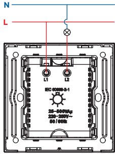
Rotary dimmer
