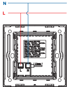
2G USB Charger, Type A+C
