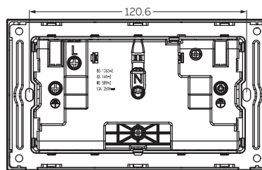
Distance between fixing screws for 2gang frames
