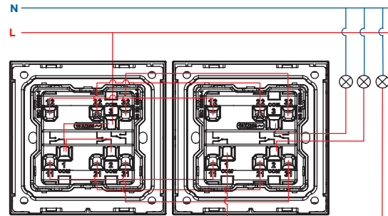
3G 2W switch
