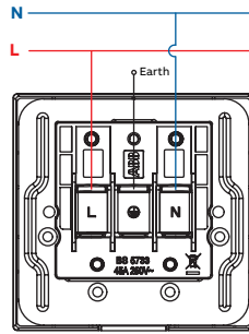
Flex outlet 45A
