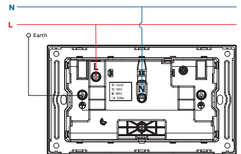
2G 13 A switched socket outlet
