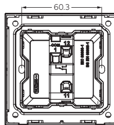
Distance between fixing screws for 1gang frames
