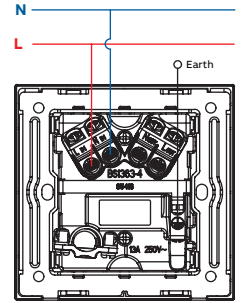
Fused connection unit
