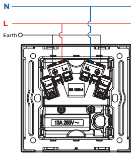
Fused switched connection unit
