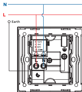
1G 13 A switched socket outlet
