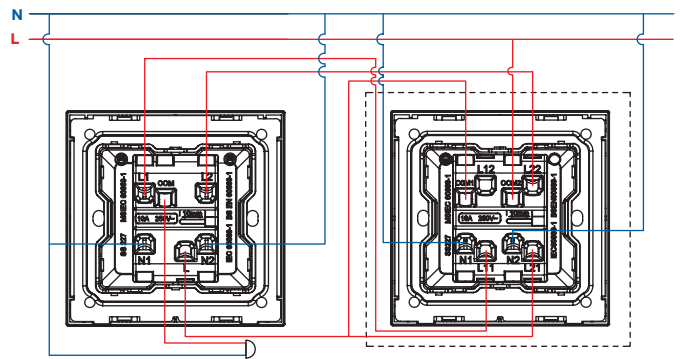
DND/MUR BELL Switch (OUTDOOR)
