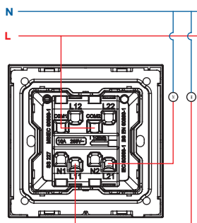
Blind Control Switch
