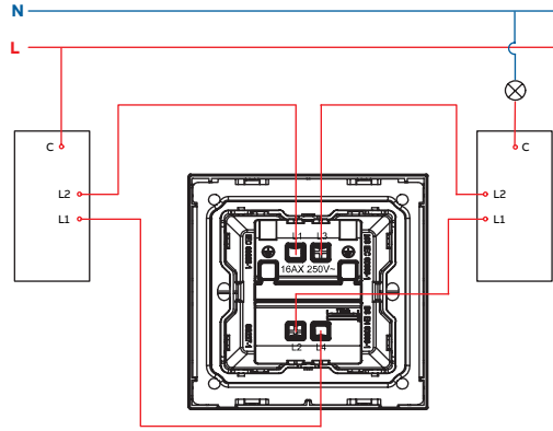
1G intermediate switch
