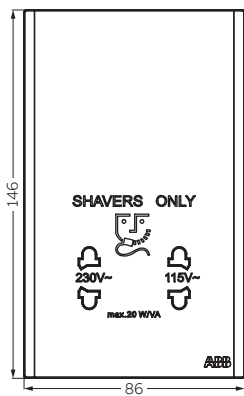
Dimensions for shaver socket
